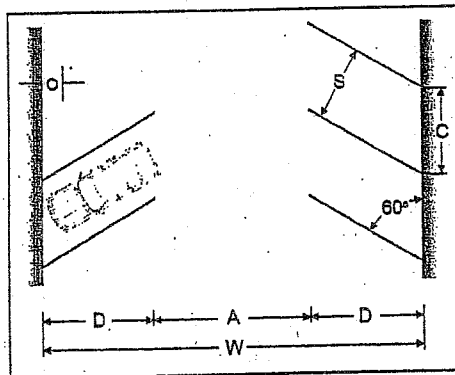
Parking Stall and Access Isle Geometry.
